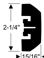
EXTRUSION
